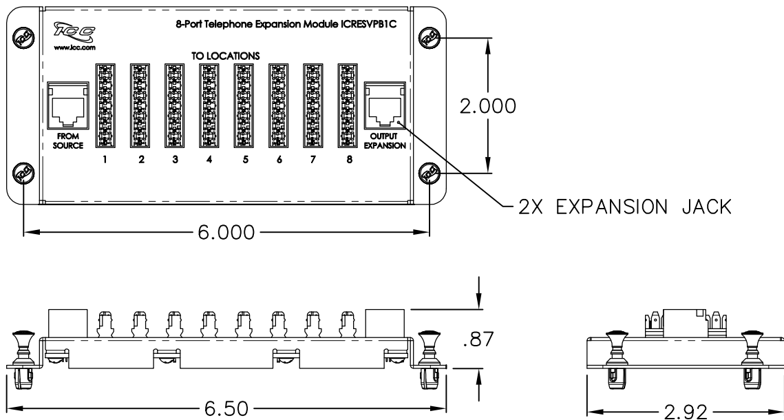
8-PORT TELEPHONE MODULE WITH EXPANSION JACKS
