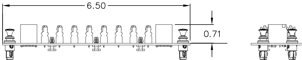
8-PORT TELEPHONE MODULE WITH EXPANSION JACKS
